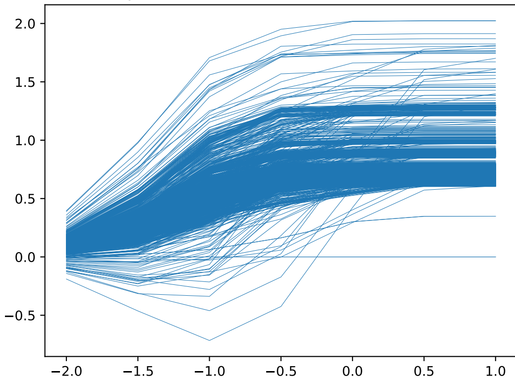
Dynamic Ricci Curvature for Geodesic 0.4
